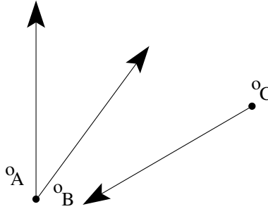
Figure 11: \mathcal{OPRA}_1^* configuration
