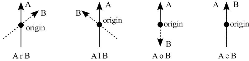
Figure 2: \mathcal{CC}_b relations
