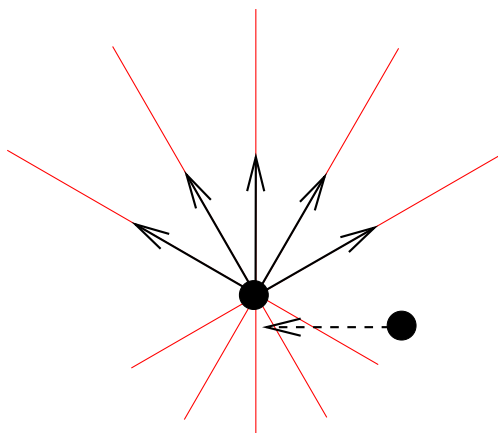
Figure 13: The OPRA_1^* relation RIGHTright+ generates all possible angles for the CYC_b relation r .
