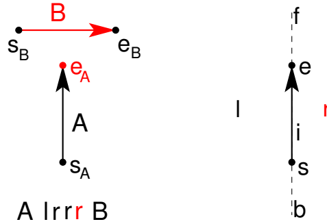
Figure 5: Orientation between two dipoles based on four dipole-point relations
