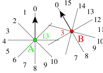
Figure 3: Two o-points in relation A \angle_{13}^3 B
