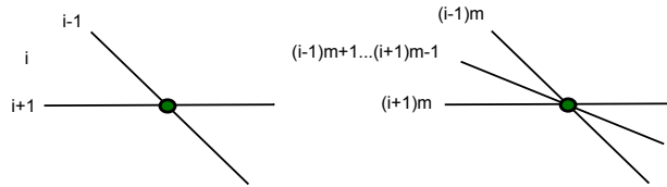
Figure 9: OPRA_n is a quotient of OPRA_{m \cdot n}
