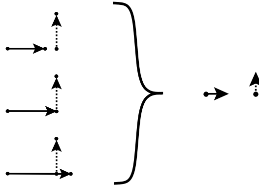
Figure 8: In a quotient homomorphism between \mathcal{DRA}_{fp} and \mathcal{OPRA}_1^* the three relations \{\text{fill}, \text{ells}, \text{illr}\} are mapped to \text{FRONTleft} .
