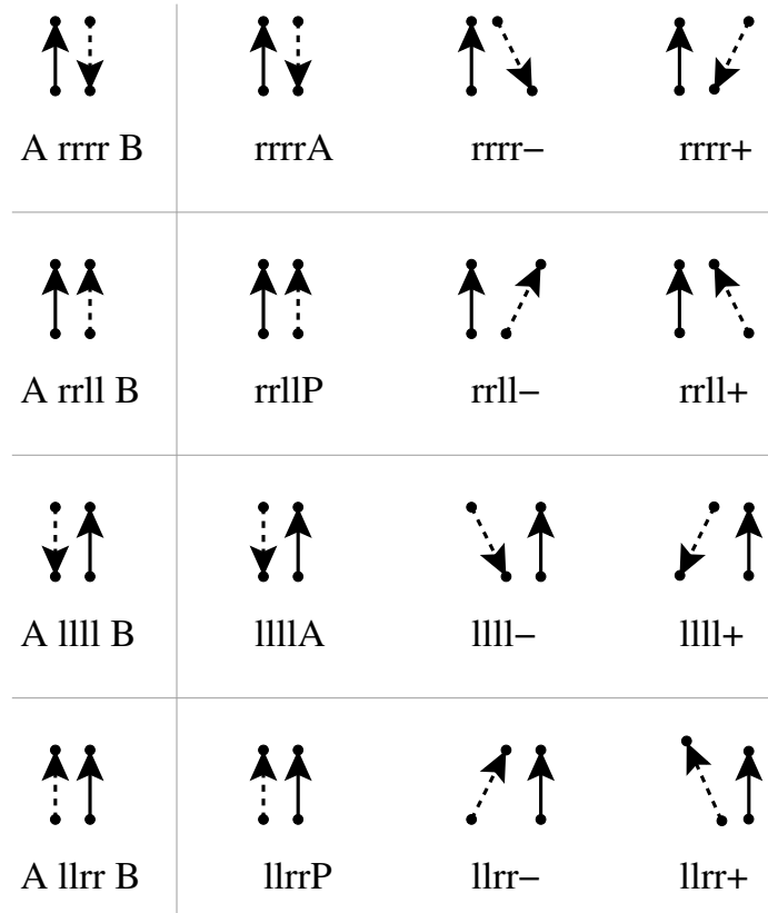
Figure 6: Refined base relations in \mathcal{DRA}_{fp}
