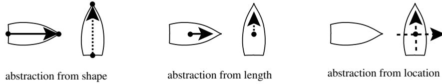
Figure 7: Modelling relative ship directions on different levels of granularity with \mathcal{DRA}_{fp} , \mathcal{OPRA}_1^* , and \mathcal{CVC}_b .
